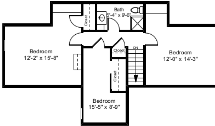
Second Floor Plan Ceiling Height = 7'-0"
