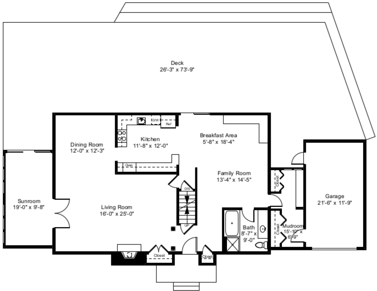
First Floor Plan Ceiling Height = 8'-0"
